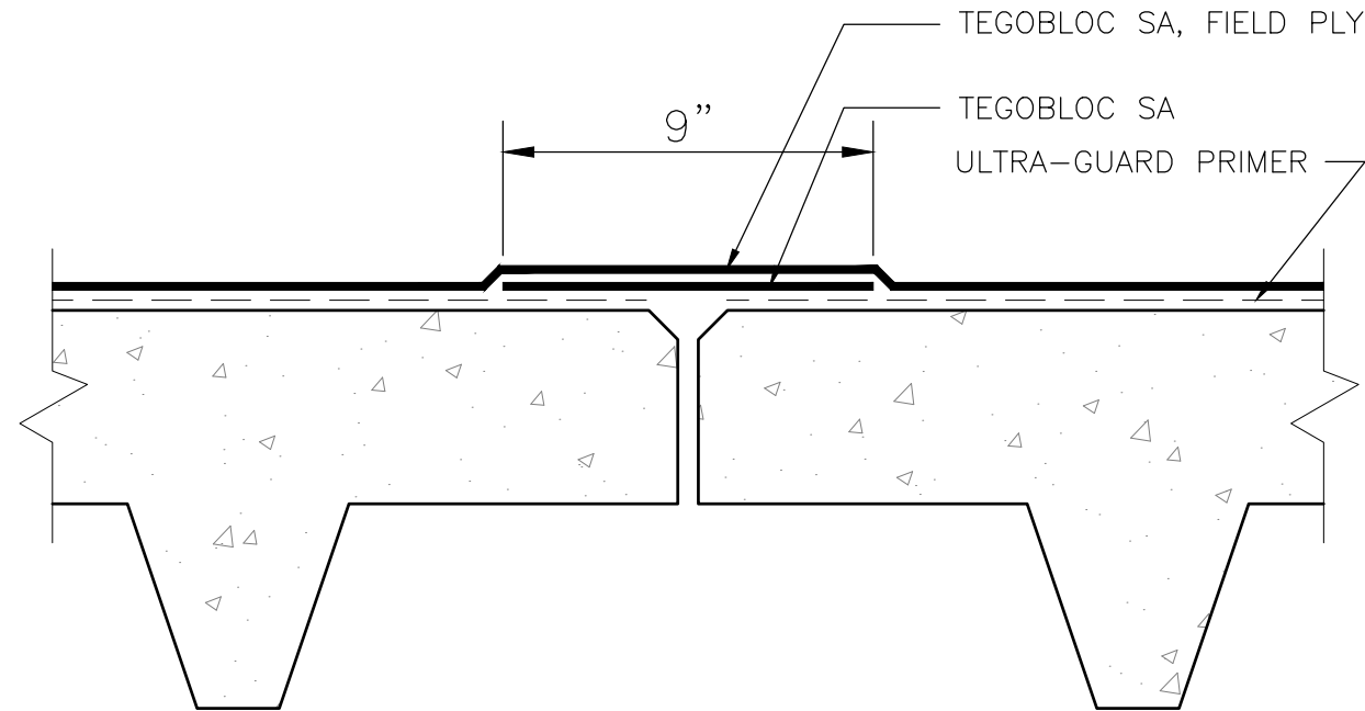
PRECAST JOINT DETAIL
