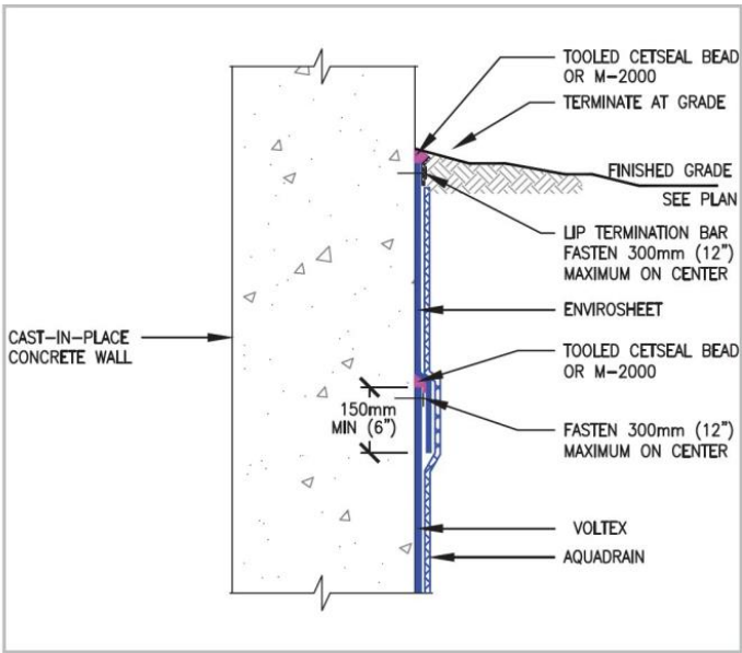
Grade Termination
